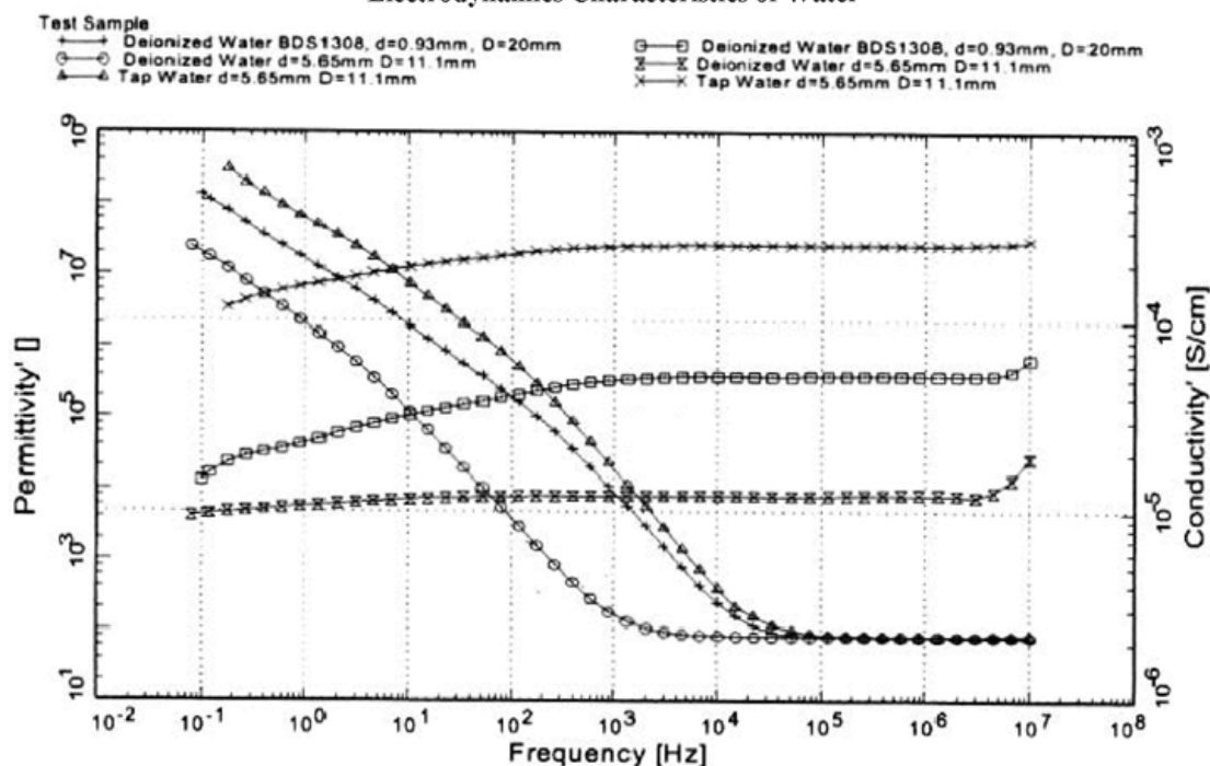
Fig 2: The relative dielectric permittivity of water significantly increases from 80 up to 10^8 and electrical conductivity of water samples decreases up to 10 times in the frequency range of 0.1 – 1000 Hz. Measurements were conducted on the samples of deionized and tap water in measurement units with different size (length and diameter) at 20°C.
