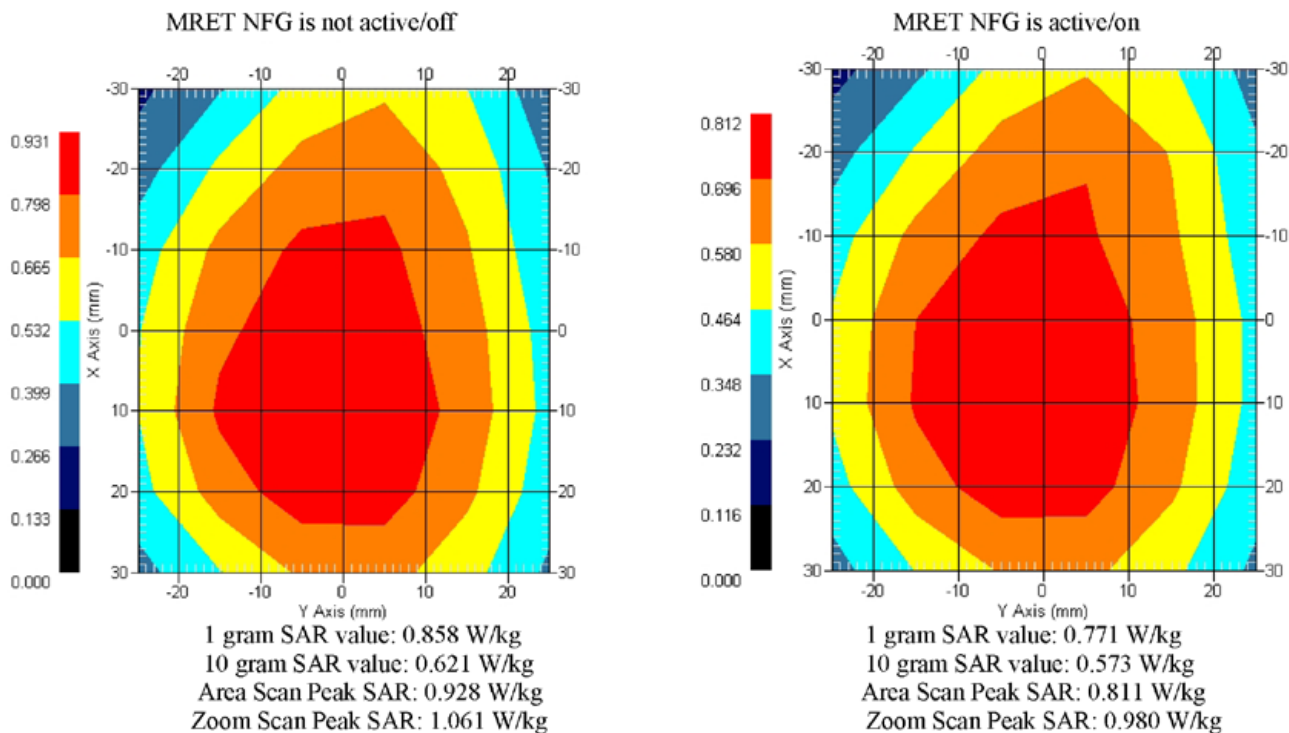
Fig 5: Phone Model: Kyocera KWC 2325; Frequency: 835.00 MHz; Max. Transmitted Power: 0.48 W; Phantom data: APREL-SAM Left Ear; Probe Sensitivity: 1.20 1.20 1.20 \mu\text{V}/(\text{V}/\text{m})^2 .
